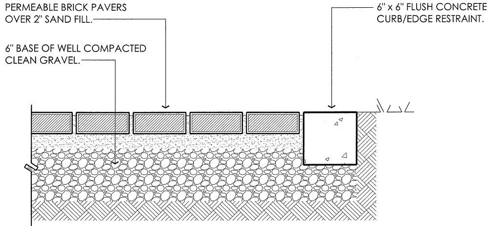
SECTION THRU PAVER EDGE - FLUSH CURB
